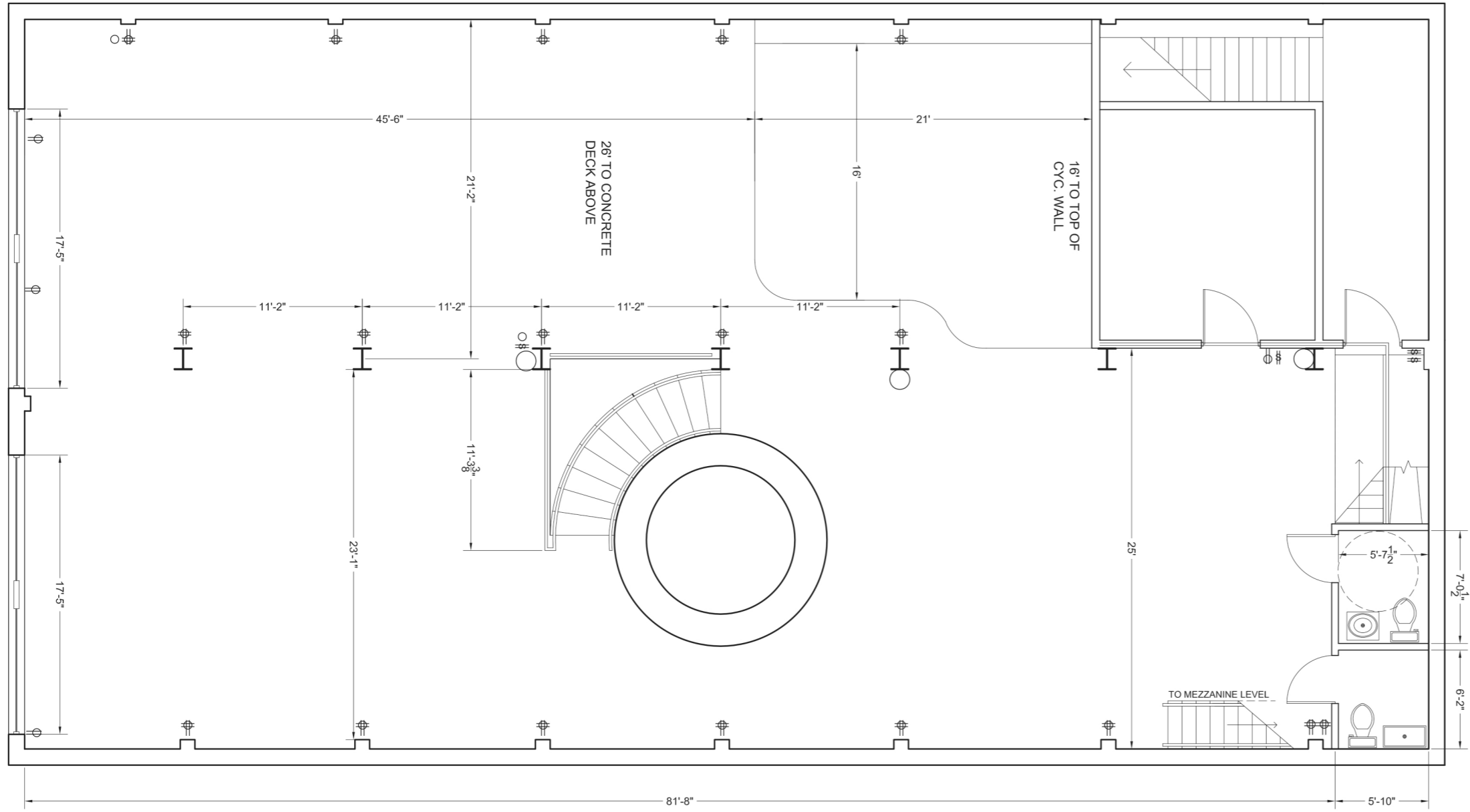
THIRD FLOOR STUDIO SCALE: 1/8"=1'-0"
